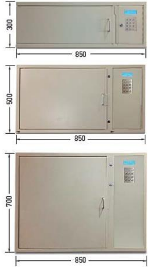
Cabinets 200mm deep
